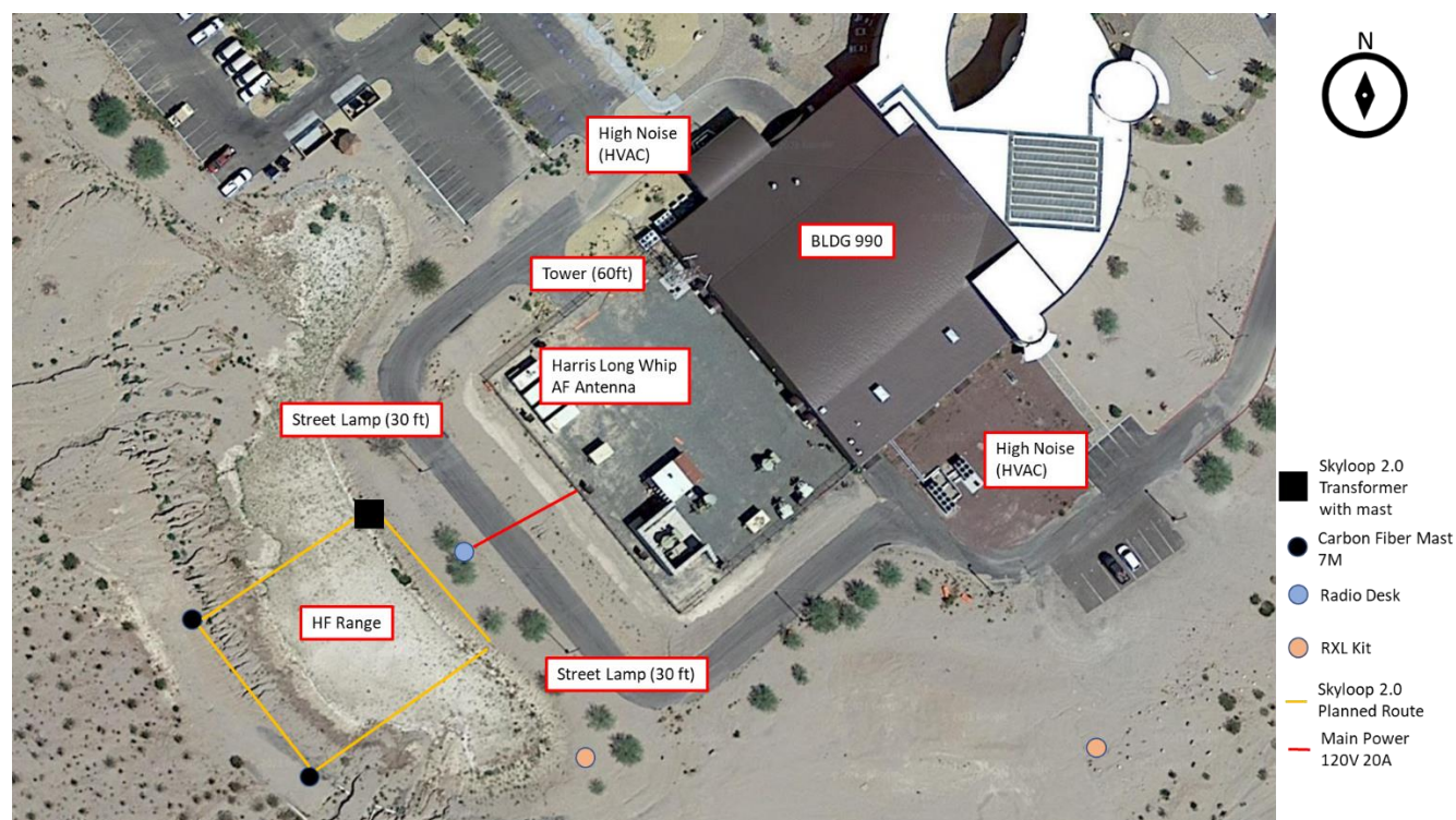
Figure 1 - Competition Station Layout w/ Skyloop 2.0
